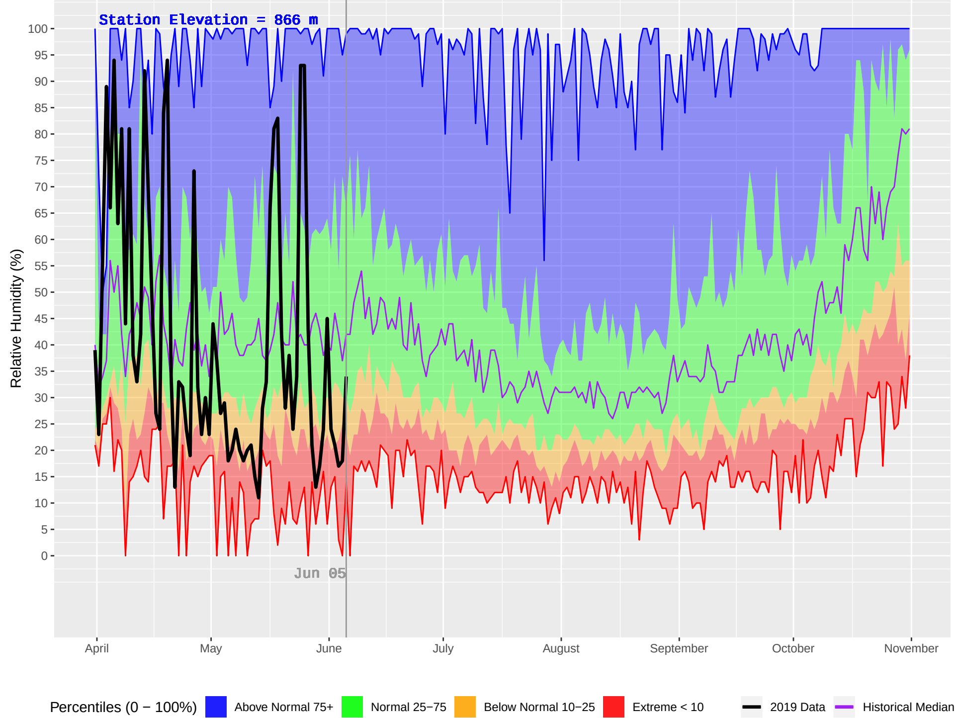
NICOLL (393) : Historical (1981–2018) and Current (2019) Daily Relative Humidity
