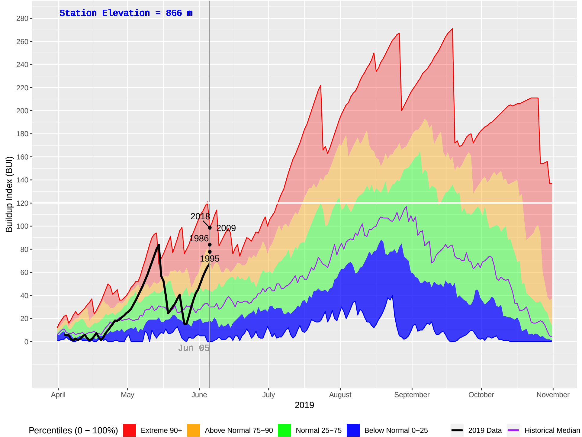
NICOLL (393) : Historical (1981–2018), Current (2019) Daily Buildup Index (BUI)
