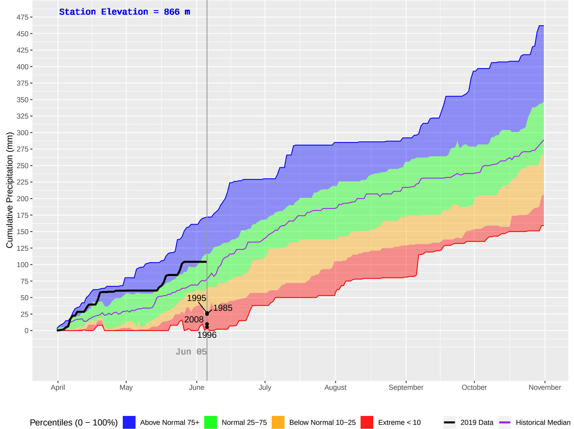
NICOLL (393) : Historical (1981–2018), Current (2019) Daily Cumulative Precipitation
