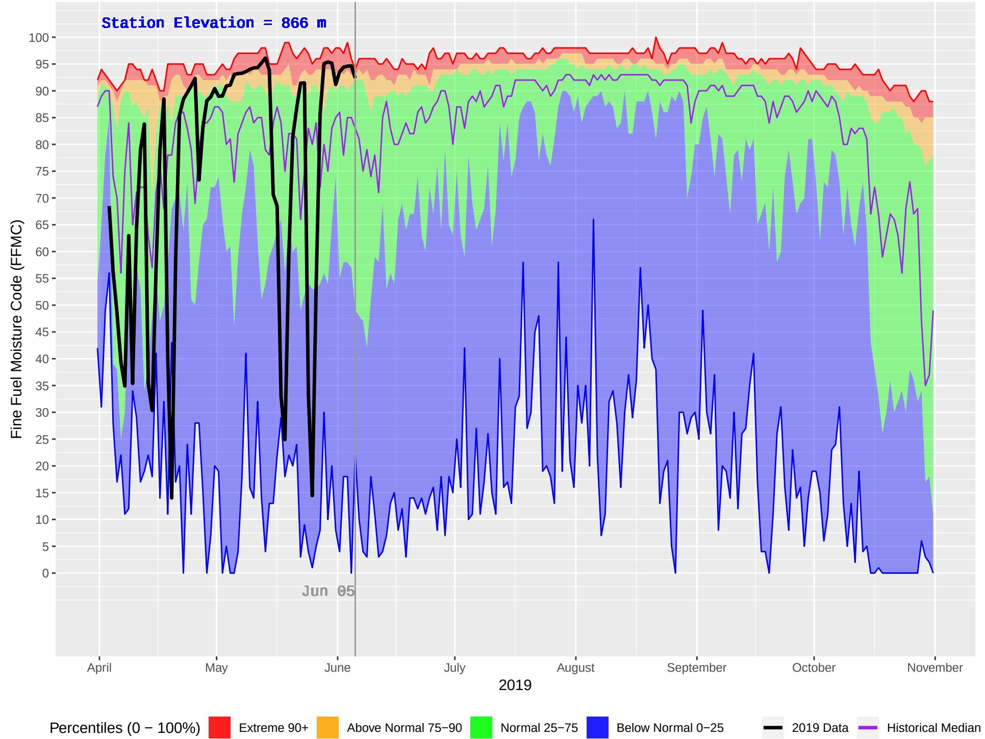
NICOLL (393) : Historical (1981–2018) and Current (2019) Daily Fine Fuel Moisture Code (FFMC)
