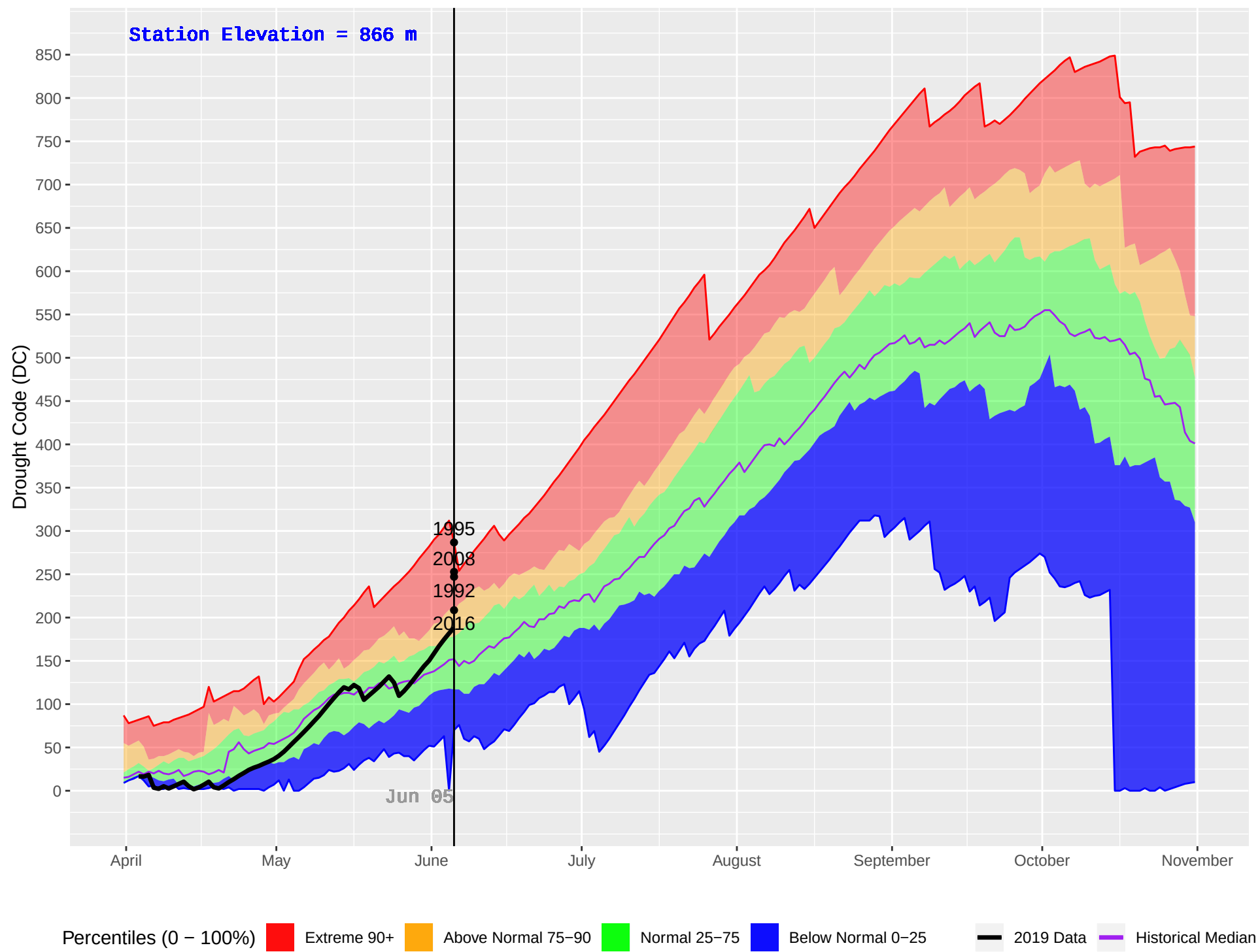
NICOLL (393) : Historical (1981–2018) and Current (2019) Daily Drought Code (DC)
