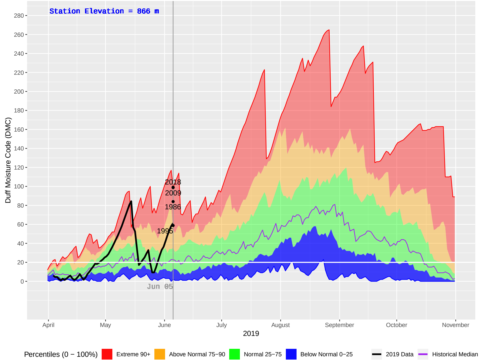
NICOLL (393) : Historical (1981–2018), Current (2019) Daily Duff Moisture Code (DMC)
